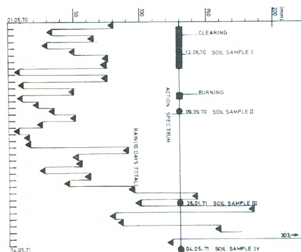
Figura 2 — Action spectrum (clearing, burning, soil sampling) and 10 days total of rainfall from May 1st, 1970 to May 4th, 1971, at SEMA-site.
